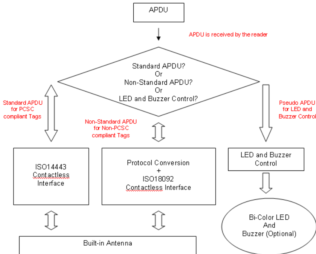
Figure 2: Basic Program Flow for Contactless Applications
